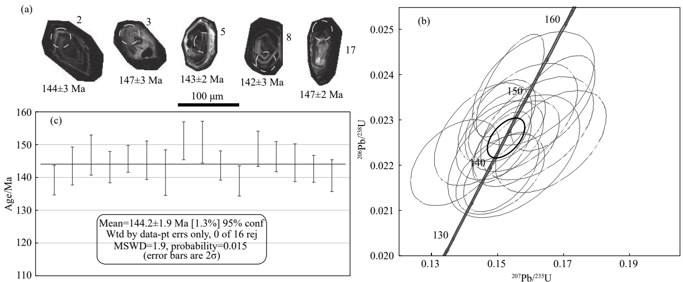
Fig. 2. Zircon CL images of spots analyzed (a), zircon U-Pb concordia diagram (b), and ^{206}\text{Pb}/^{238}\text{U} weighted mean age (c) of the pegmatite vein in Dahongliutan lithium deposit.
