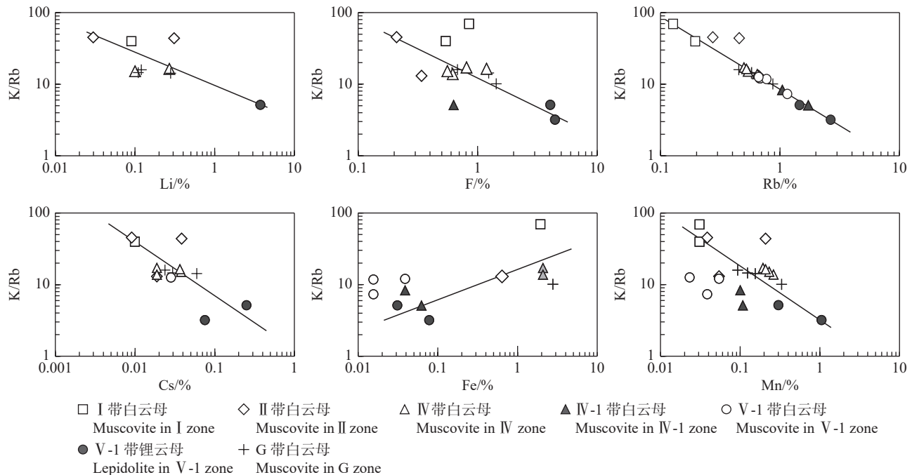
图 5 Manono-Kitotolo 伟晶岩中云母的 K/Rb vs. Li、F、Rb、Cs、Fe、Mn 相关图解(Li 数据来源于 Dewaele et al., 2016; Rb、Cs、Fe、Mn 元素含量根据表 1 中氧化物的含量换算) Fig.5 K/Rb vs. Li, F, Rb, Cs, Fe, Mn for micas in the Manono-Kitotolo pegmatite (Li data after Dewaele et al., 2016; F, Rb, Cs, Fe, Mn contents are converted according to the oxide content in Table 1)
