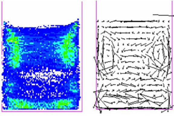
图 6 PEPT 研究立式搅拌细磨装备中介质运动状态 Fig. 6 Media state in vertical stirring grinding equipment using PEPT
