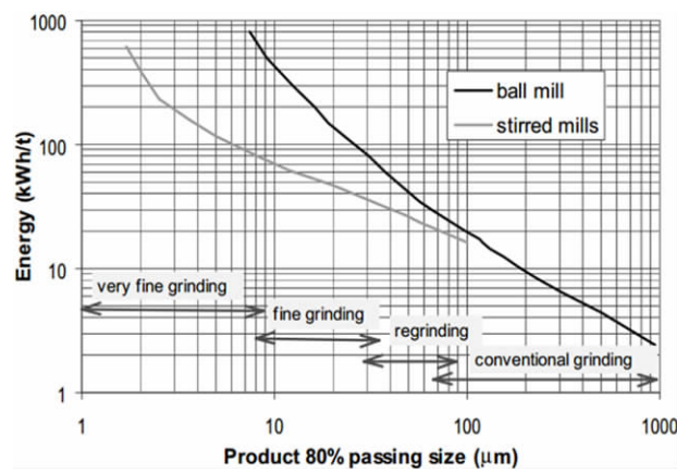
图 1 不同磨矿阶段的球磨机和搅拌细磨装备能耗对比 Fig. 1 Comparison of energy consumption between stirring mill and ball mill in different grinding stages
