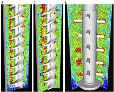
图 5 立式细磨装备介质速度分布情况 Fig. 5 Distribution of media velocity state of vertical grinding equipment
