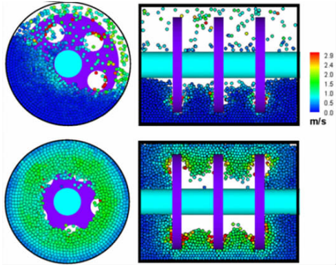
图 4 搅拌细磨装备内部介质运动状态分布情况 Fig. 4 Distribution of media motion state in stirring grinding equipment
