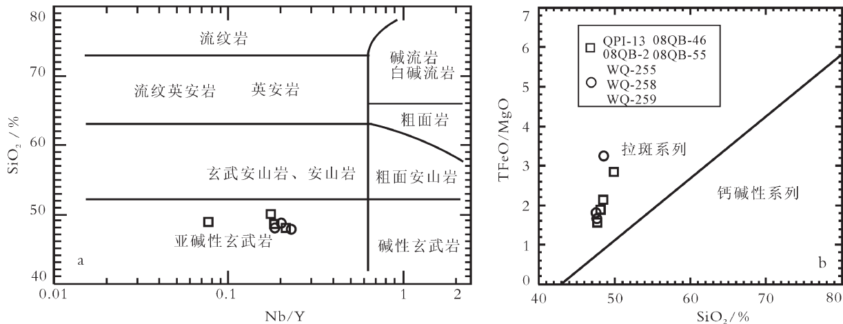
图 5 东沟蛇绿岩的基性火山岩 \text{SiO}_2\text{-Nb/Y} 和 \text{TFeO/MgO-SiO}_2 图解(底图分别据参考文献[16]和[17]) Fig. 5 \text{SiO}_2\text{-Nb/Y} and \text{TFeO/MgO-SiO}_2 diagrams of basic volcanic rocks from Donggou ophiolites
