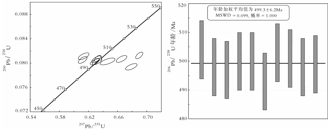
图 4 东沟蛇绿岩基性火山岩锆石 U-Pb 谐和图和年龄加权平均图 Fig. 4 Zircon concordia diagram of basic volcanic rocks in Donggou ophiolites
