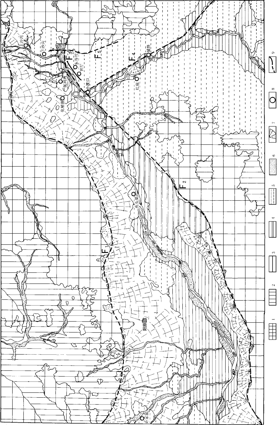
图 1 泥河湾盆地地貌与活动断裂图 Fig. 1 Geomorphological units and active faults in Nihewan Basin
