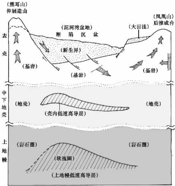
图 3 泥河湾盆地盆山耦合 响应理论模型图（据邢作云等 2005 [10] 修改） Fig.3 Theoretical model of basin-mountain coupling response for the Nihewan Basin (Modified from Xing Zuo-yun et al 2005 [10] )
