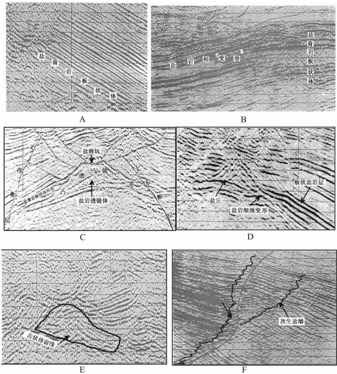
图 3 东濮凹陷文留油田盐岩地震反射特征 Fig 3 Seismic reflection feature of halite in the Dongpu depression of the Wenliu oilfield
