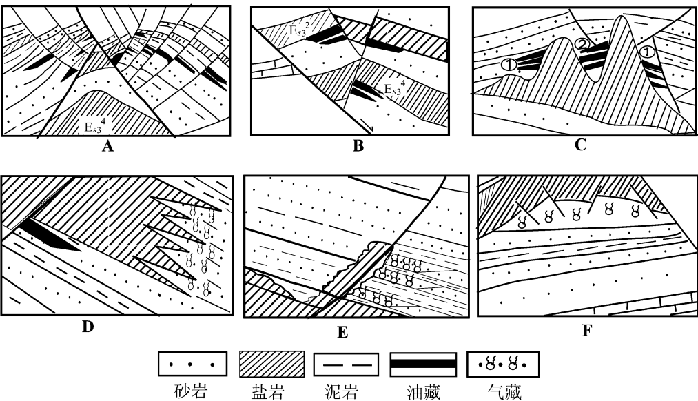
图 4 与盐岩相关的油气藏的类型 Fig 4 Hydrocarbon reservoir types relating to halite
